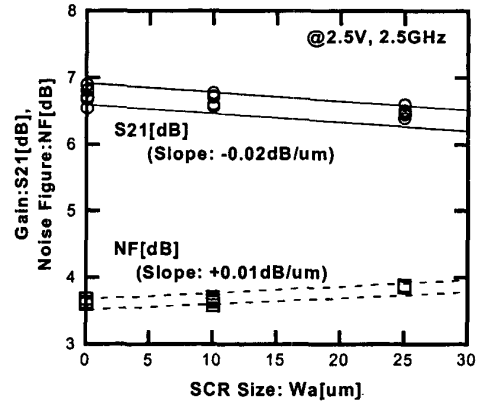
Fig. 9: Measured SCR Size effects on S_{21} and NF in the LNA. (Measurement: 5 points per each size)
