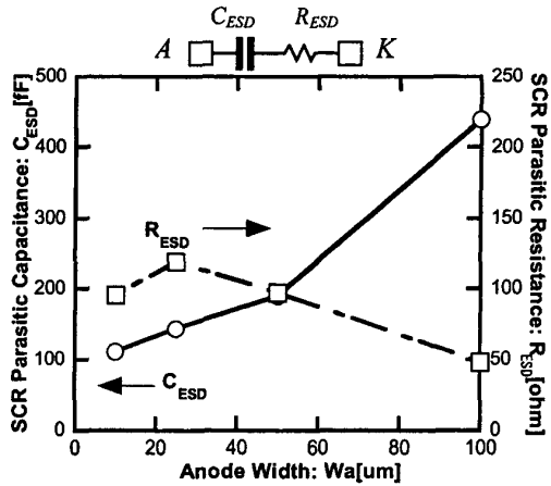
Fig. 4: SCR size effect on the equivalent circuit capacitance ( C_{ESD} ) and resistance ( R_{ESD} ) of ESD protection device as extracted from the S-parameter of the unit SCR in the 0.1-10GHz frequency range.
