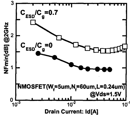
Fig. 6: Measured effect of input ESD protection device capacitance ( C_{ESD} ) on the NMOSFET NF_{min} -vs- I_d . V_{b2}
