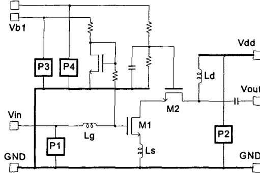
Fig. 7: Schematic of the ESD-protected LNA circuit. P1-P4 indicate the SCR-based ESD protection devices.
